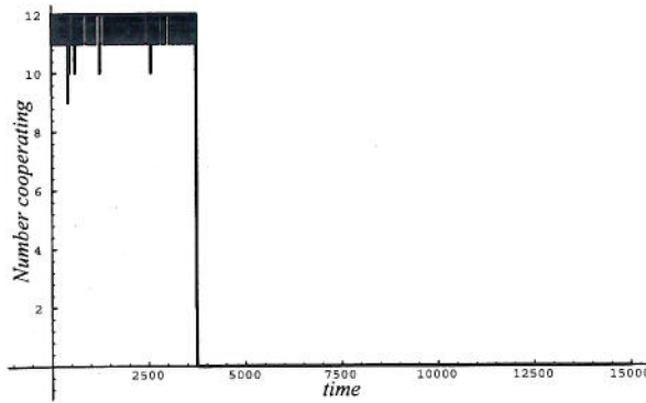
Fig. 5. Outbreak of defection. At t = 0 , two cooperating groups of size n = 6 merge to form a larger, cooperating group of size n = 12 . The agents follow bandwagon expectations and have horizon length H = 9.5 throughout, with p = 0.93 , b = 2.5 , c = 1 , \alpha = 1 and \tau = 1 . For these parameters, cooperation is the optimal state for a group of size n = 6 , but for the combined group of size n = 12 , cooperation is metastable. Indeed, as the figure shows, metastable cooperation persists for almost 4,000 time steps in this example. Uncertainty ( p less than one) ensures that eventually a large fluctuation in the perceived number of agents cooperating eventually takes the group over into a state of mutual defection, which is optimal.
