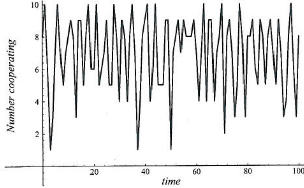
Fig. 8. Oscillatory dynamics of a group of opportunistic agents of size n = 10 . The agents have horizon length H = 10 , with p = 0.99 , reevaluation rate \alpha = 1 , information delay \tau = 1 , and the same benefit and cost for cooperation as before.
