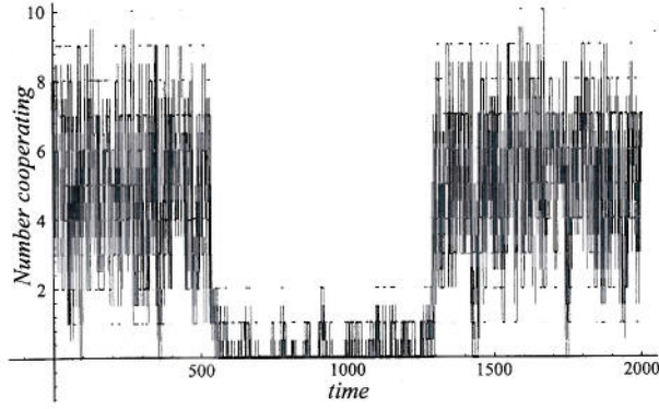
Fig. 9. Bursty stable and chaotic dynamics of a group of opportunistic agents of size n = 10 . The agents have horizon length H = 5.5 , with p = 0.9 , reevaluation rate \alpha = 1 , information delay \tau = 4 , and the same benefit and cost for cooperation as before. The flip-flops between the two attractors of chaotic oscillations and the fixed point at overall defection extend into time beyond the time series shown here.
