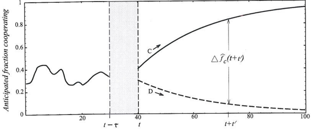
Fig. 2. Agents extrapolate the evolution of the group's behavior using delayed information of the fraction cooperating. The upper curve represents how a member expects the dynamics to evolve if he cooperates, the lower if he defects. The rate with which the two curves respectively rise and fall depends on the members' class of expectations functions. Agents with bandwagon expectations extrapolate out very flat curves when the fraction cooperating is small and much steeper curves when this fraction is large. Opportunistic agents, in contrast, extrapolate out very flat curves whenever the fraction cooperating becomes either small or large, but predict sharper rises and declines for intermediate levels of cooperation.
