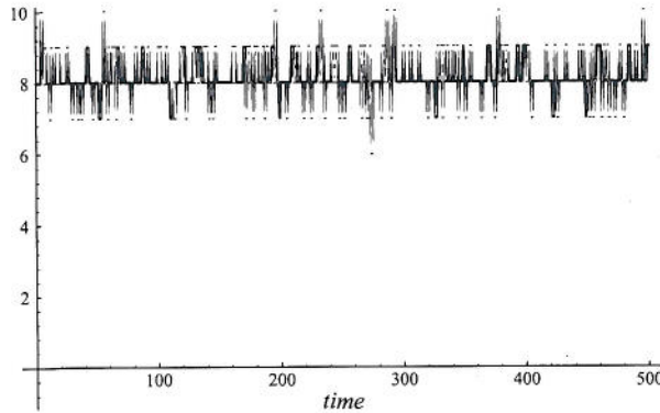
Fig. 6. Fluctuations about the mixed cooperative/defecting fixed point for an opportunistic group of size n = 10 , horizon length H = 10 , with p = 0.95 . The number cooperating fluctuates around n = 8 and the typical size of fluctuations is \pm 1 with an occasional fluctuation of size two.
