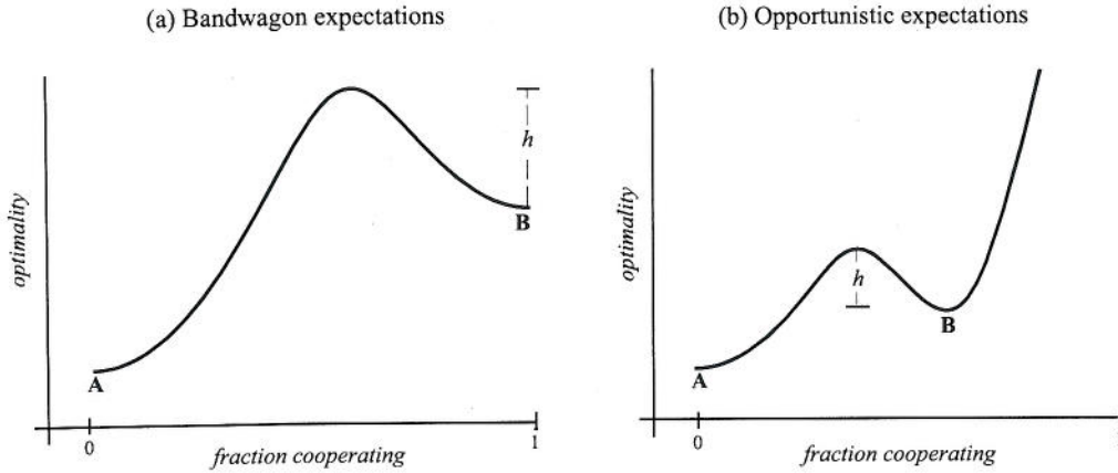
Fig. 4. The optimality function \Omega vs. f_c , the fraction of agents cooperation, for bandwagon expectations in (a) and opportunistic expectations in (b). The global minimum is at A, local minimum at B, and h is the height of the barrier separating state B from A.
