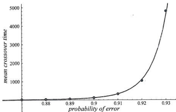
Fig. 7. Exponential increase of crossover time as a function of the probability p that an agent's action is misperceived. The mean crossover time was obtained by averaging over 600 simulations at each value of the uncertainty parameter p . In all the runs, n = 12 , H = 9.5 , b = 2.5 , c = 1 , \alpha = 1 and \tau = 1 , with bandwagon expectations. The gray curve is an exponential fit to the data.
