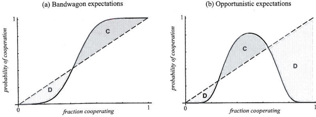
Fig. 3. The fixed points of the differential equation describing the dynamics of group cooperation are given by the intersection of y = \rho_c(f_c) and y = f_c . In region C where \rho_c(f_c) > f_c , the dynamics evolves towards more cooperation, while in region D where f_c > \rho_c(f_c) , the dynamics evolves towards more defection. Contrasting (a) and (b) hints at the difference in the dynamical behavior for bandwagon vs. opportunistic expectations. For opportunistic expectations, the more cooperative fixed point occurs where \rho_c(f_c) intersects f_c with a negative slope. When the slope at this point of intersection is steep enough, the fixed point becomes unstable causing oscillations and chaos, behavior that is not observed for bandwagon expectations.
